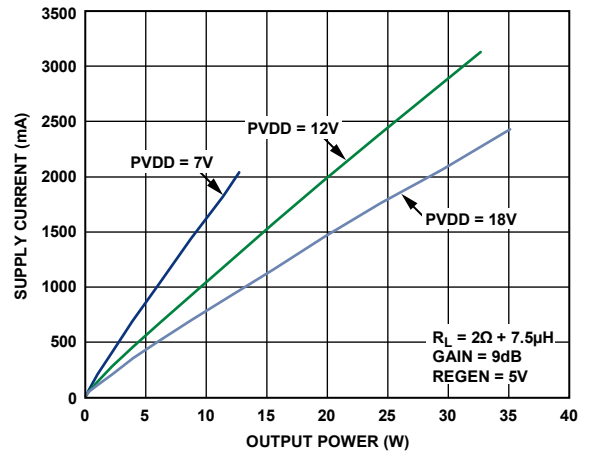
Figure 25. Supply Current vs. Output Power into 2Ω; Mono Mode; PVDD = 7V, PVDD = 12V, PVDD = 18V
