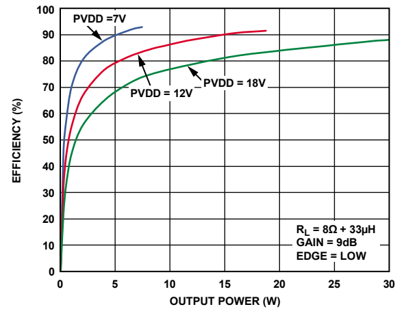
Figure 26. Efficiency vs. Output Power into 8Ω; PVDD = 7V, PVDD = 12V, PVDD = 18V
